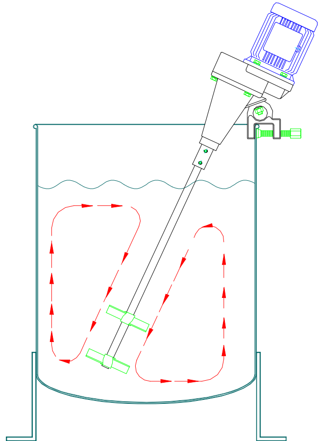
Typical Mixer Installation
